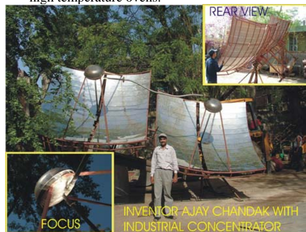
Photograph 2: 'Industrial Solar Concentrator' for hot air up to 200°C
